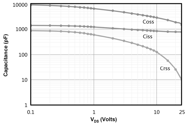
Figure 8: Capacitance Characteristics
