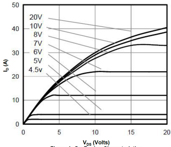
Figure 1: On-Region Characteristics
